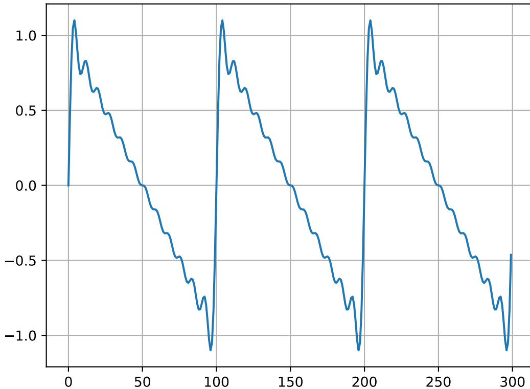
Sawtooth, 12 harmonics
