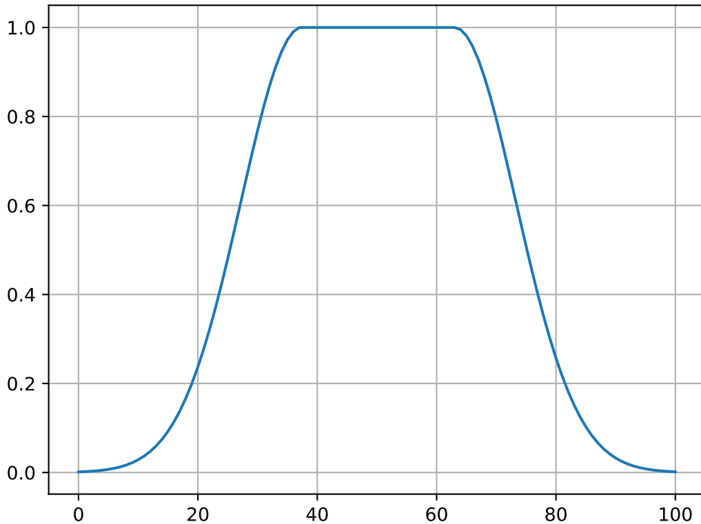
A Fat Gaussian Curve
