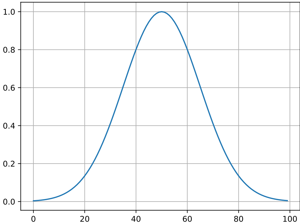
A Gaussian Curve
