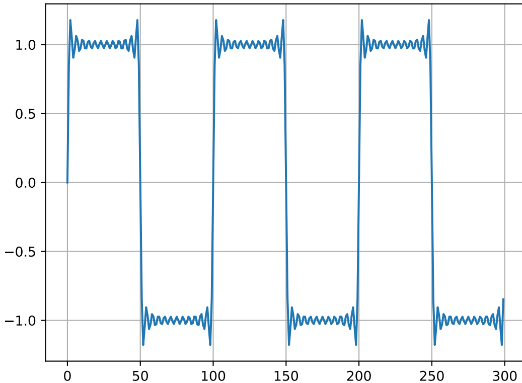
Square wave, 12 harmonics
