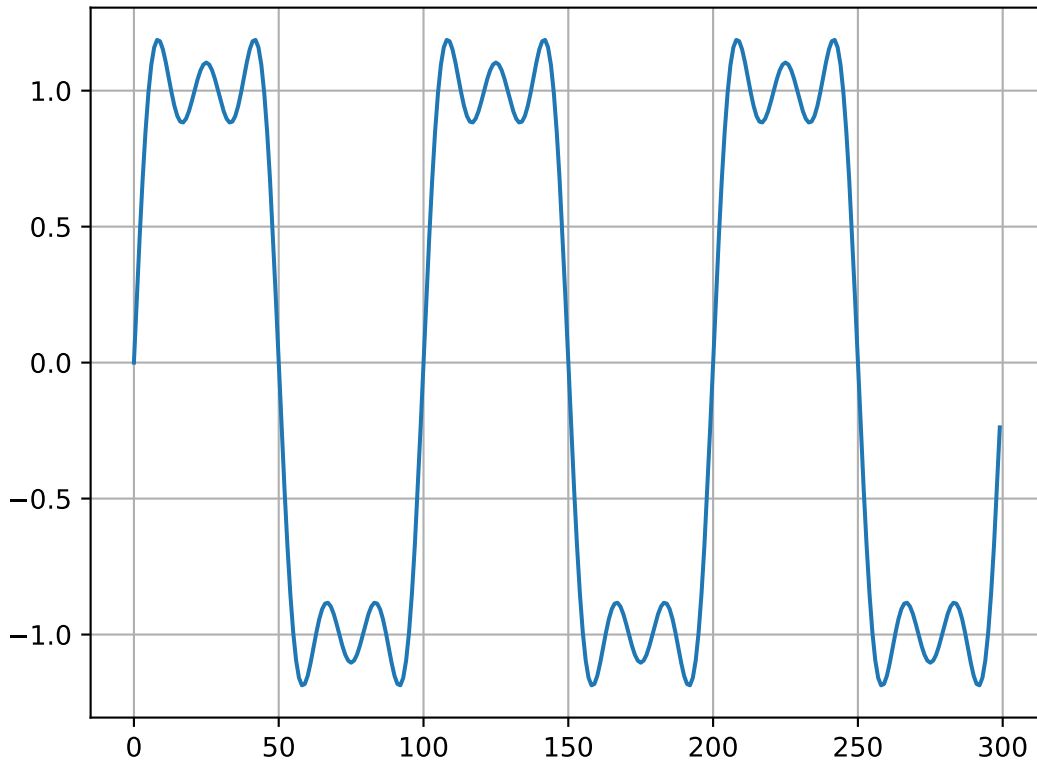
Square wave, 3 harmonics
