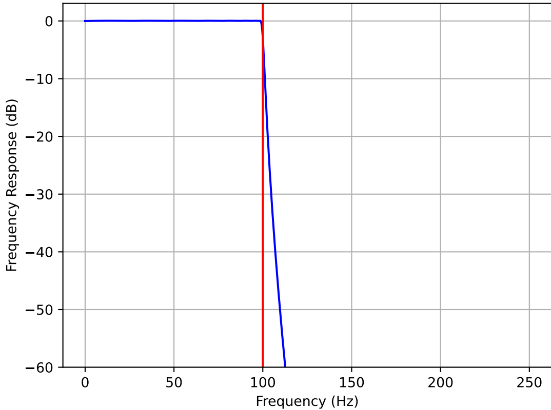
Low Pass IIR Frequency Response order = 15, f_c = 100.0 Hz, sr = 500.0 Hz
