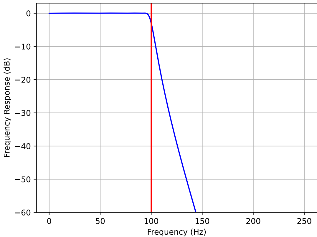
Low Pass IIR Frequency Response order = 7, f_c = 100.0 Hz, sr = 500.0 Hz
