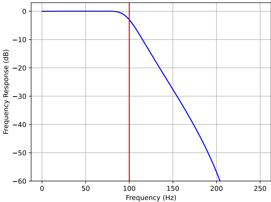
Low Pass IIR Frequency Response order = 3, f_c = 100.0 Hz, sr = 500.0 Hz
