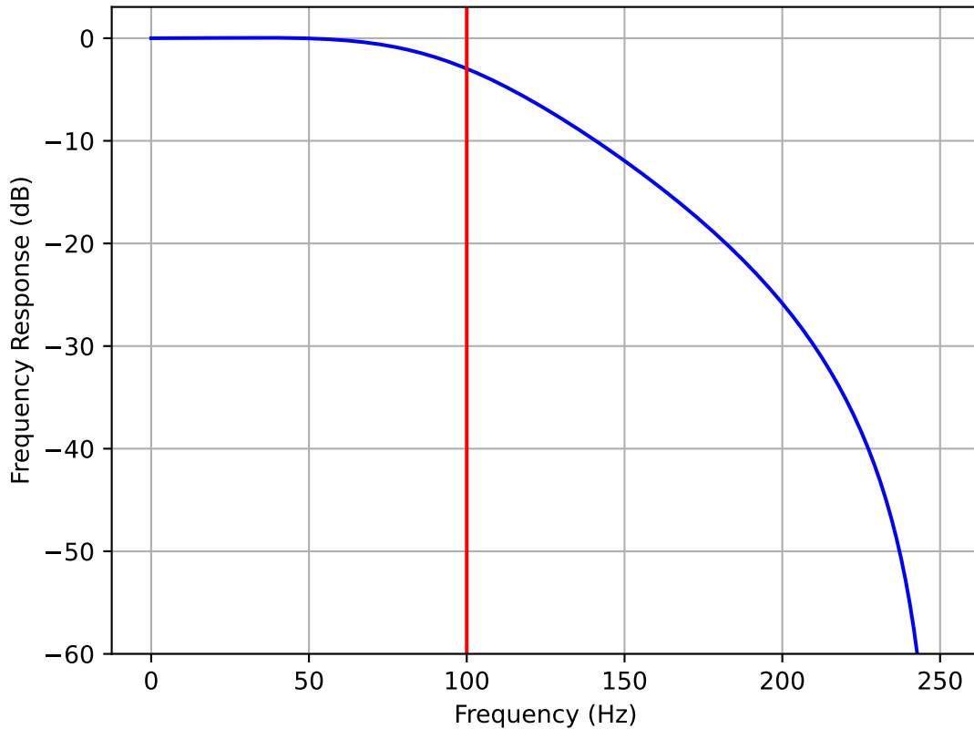
Low Pass IIR Frequency Response order = 1, f_c = 100.0 Hz, sr = 500.0 Hz
