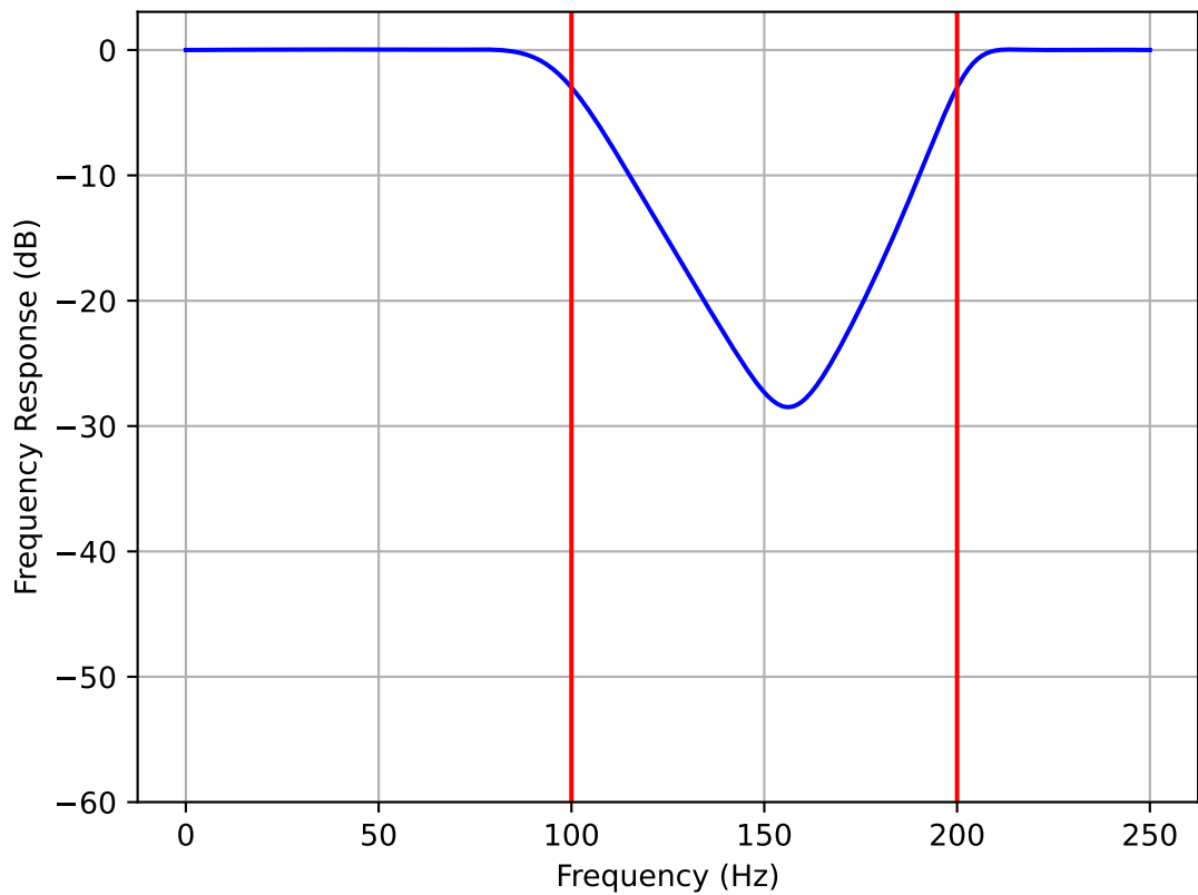
Band Reject IIR Frequency Response order = 3, fl = 100.0 Hz, fl = 200.0 Hz, sr = 500.0 Hz
