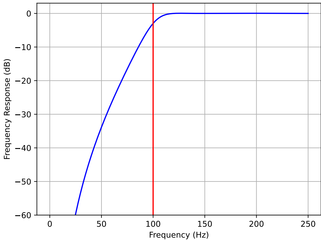
High Pass IIR Frequency Response order = 3, f_c = 100.0 Hz, sr = 500.0 Hz
