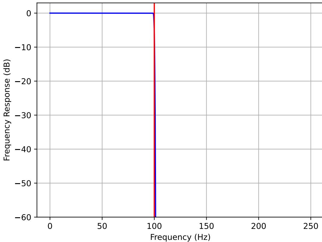
Low Pass FIR Frequency Response order = 1024, f_c = 100.0 Hz, sr = 500.0 Hz
