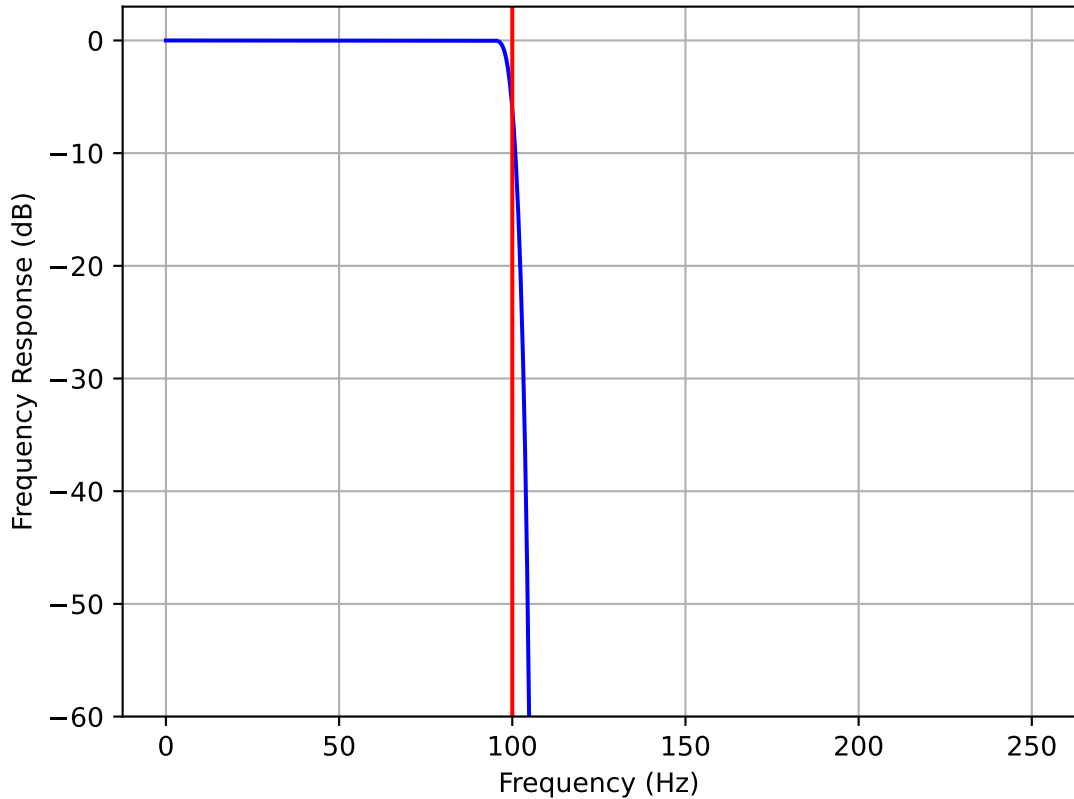
Low Pass FIR Frequency Response order = 256, f_c = 100.0 Hz, sr = 500.0 Hz
