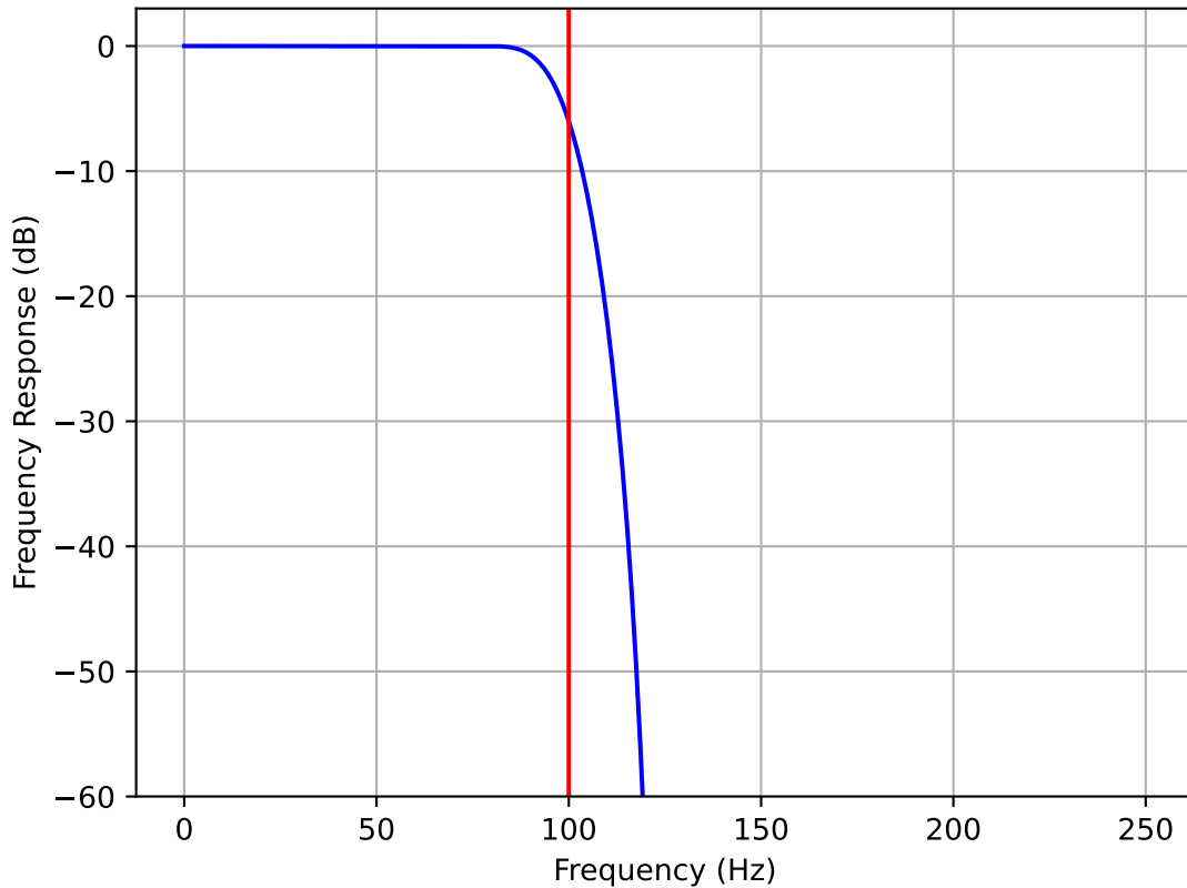
Low Pass FIR Frequency Response order = 64, f_c = 100.0 Hz, sr = 500.0 Hz
