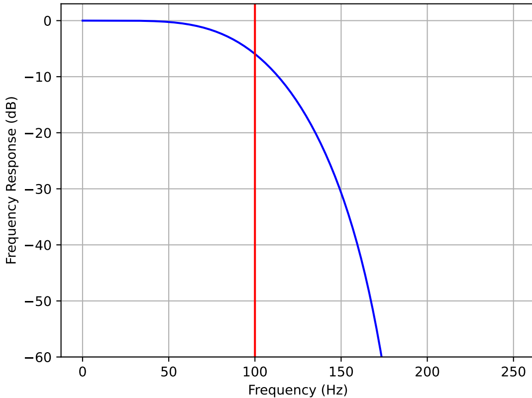
Low Pass FIR Frequency Response order = 16, f_c = 100.0 Hz, sr = 500.0 Hz
