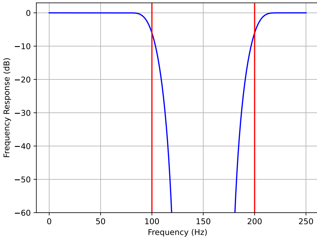
Band Reject FIR Frequency Response order = 64, fl = 100.0 Hz, fl = 200.0 Hz, sr = 500.0 Hz
