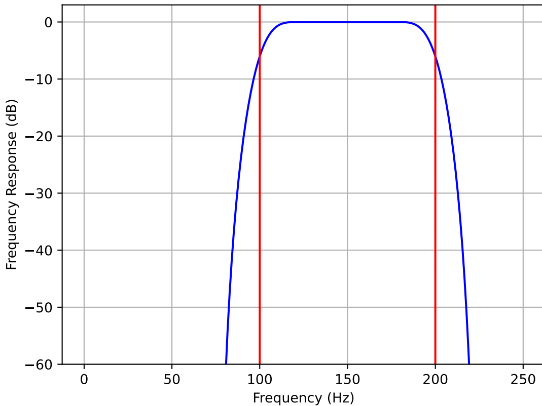
Band Pass FIR Frequency Response order = 64, fl = 100.0 Hz, fl = 200.0 Hz, sr = 500.0 Hz
