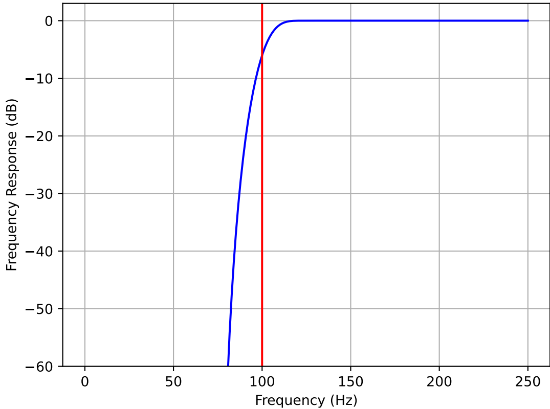
High Pass FIR Frequency Response order = 64, f_c = 100.0 Hz, sr = 500.0 Hz
