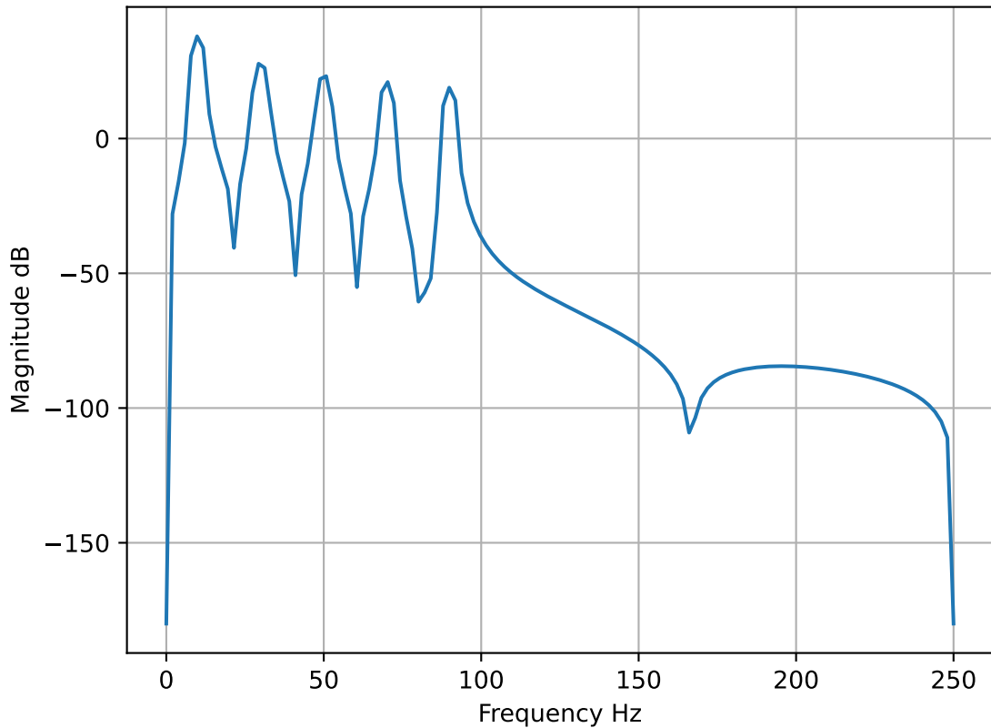
Frequency Domain, With Hanning Window
